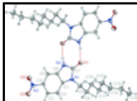
Fig. 1. Thermal ellipsoid plot (Barbour, 2001) of two molecules of C 15 H 21 N 3 O 3 disposed about a center of inversion: drawn at the 50% probability level.
